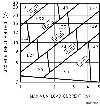
FIGURE 4. LM2678-5.0
