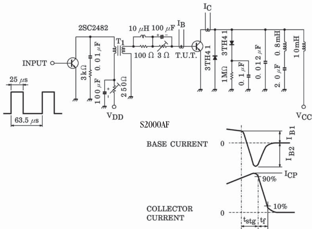
Fig.1 SWITCHING TIME TEST CIRCUIT
